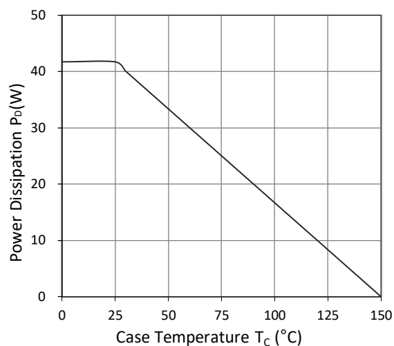
Figure 9. Power Dissipation
