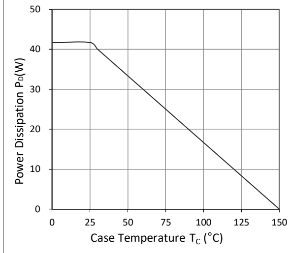
Figure 9. Power Dissipation
