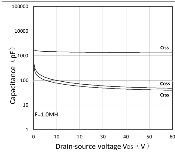
Figure 7. Capacitance Characteristics
