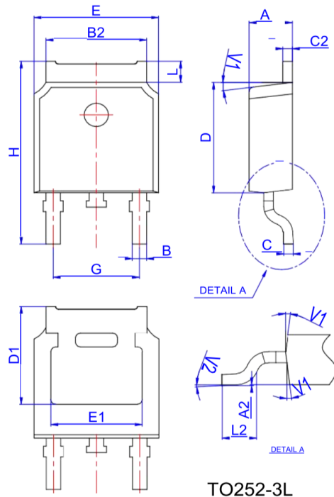
TO252-3L
