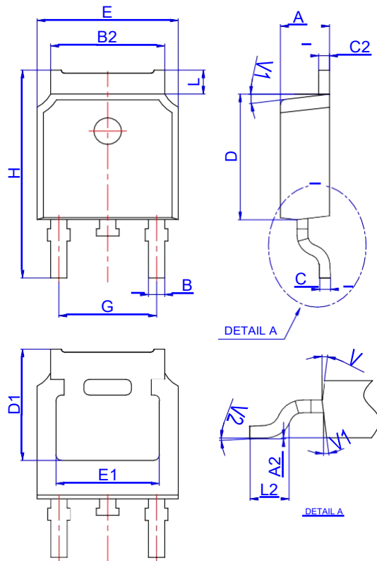
TO252-3L
